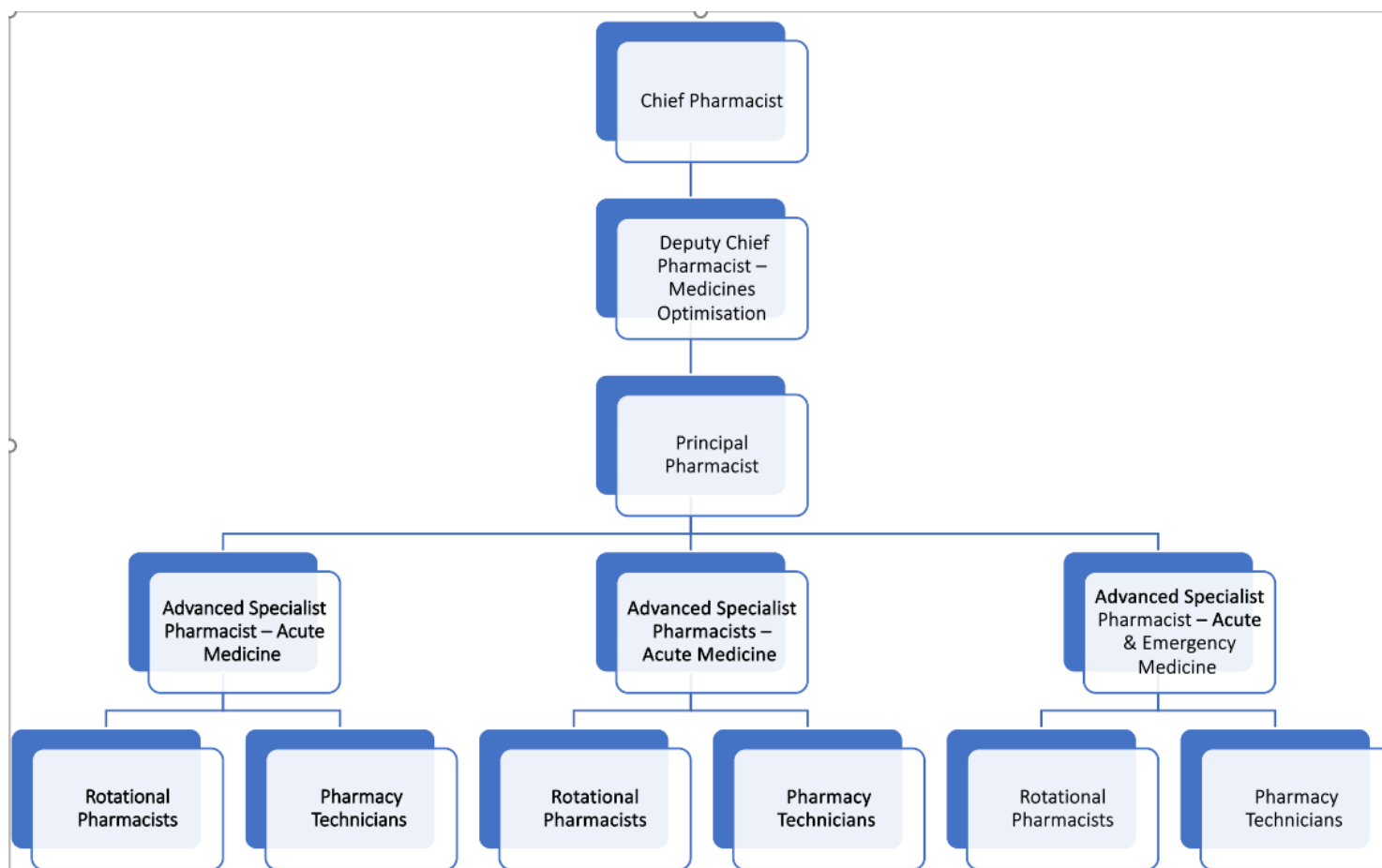
Structure Chart
